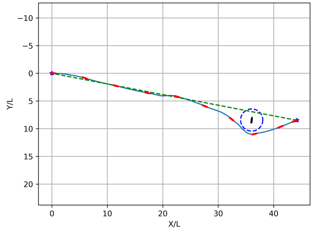
FIGURE 14: Dynamic Obstacle Case 2.
